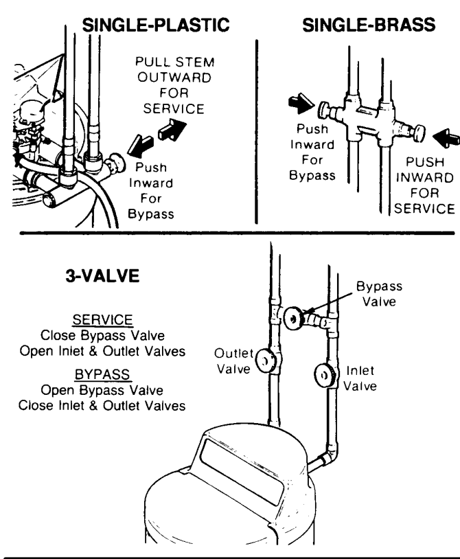
FIG. 16 BYPASS VALVES
